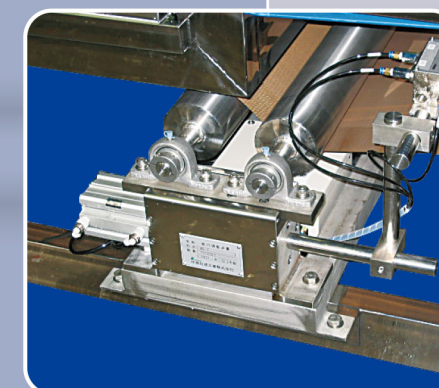
蛇行防止装置 BELT TRAINING SYSTEM
